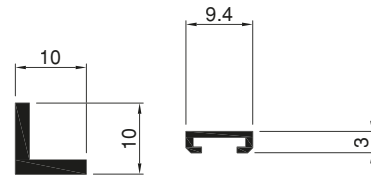
Art.Nr. A8110 L - Winkelprofil 10x10x2
